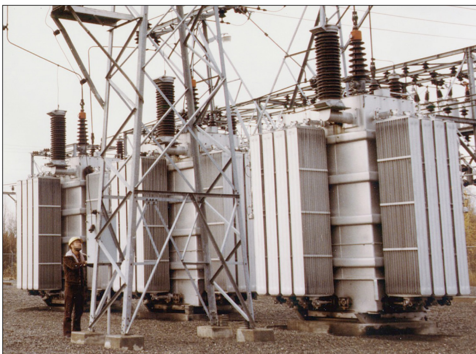
Figure 2: Large Power Transformers
